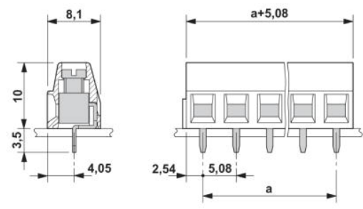
Dimensioned drawing
